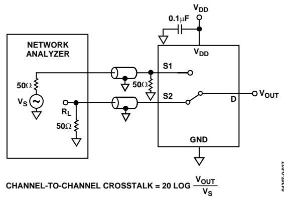
Figure 27. Channel-to-Channel Crosstalk
