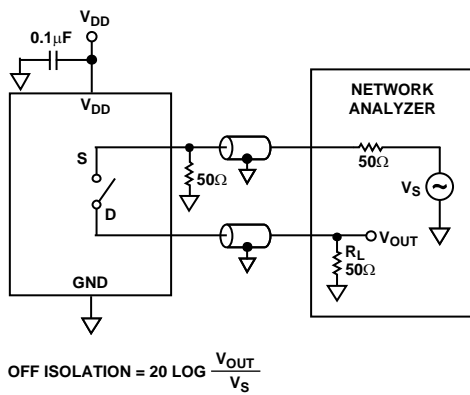
Figure 25. Off Isolation
